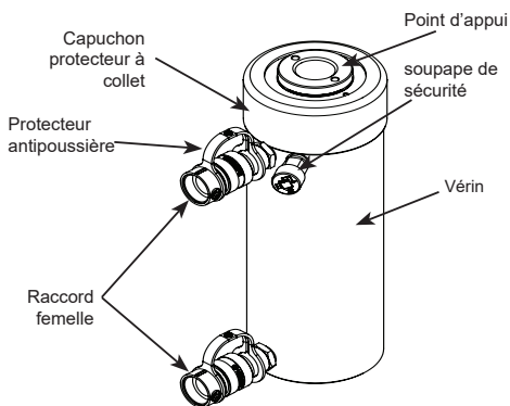
Figure 1 - Composants de vérin type
