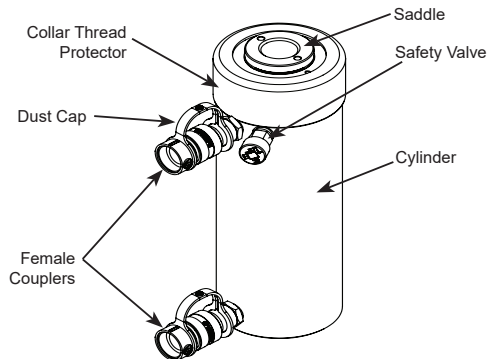
Figure 1 - Typical Cylinder Components
